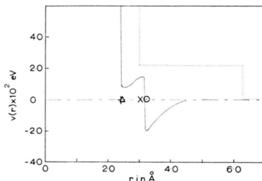
Fig. 3. Interatomic potentials, v(r) . \cdots Ledge potential [4]. \text{—} Sketch of proposed potential for Bi. \times \sigma_A^{\text{Sn}} + \sigma_B^{\text{Sn}} ; \circ \sigma_A^{\text{Bi}} , \Delta \sigma_B^{\text{Bi}} .
